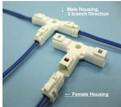
CA01 Series 2 pins in 3 branch direction
