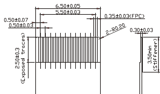
FPC Dimensions
