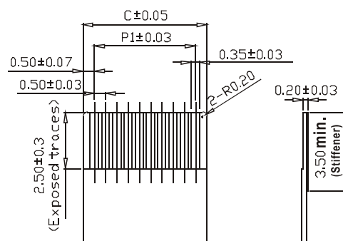
FPC Dimensions
